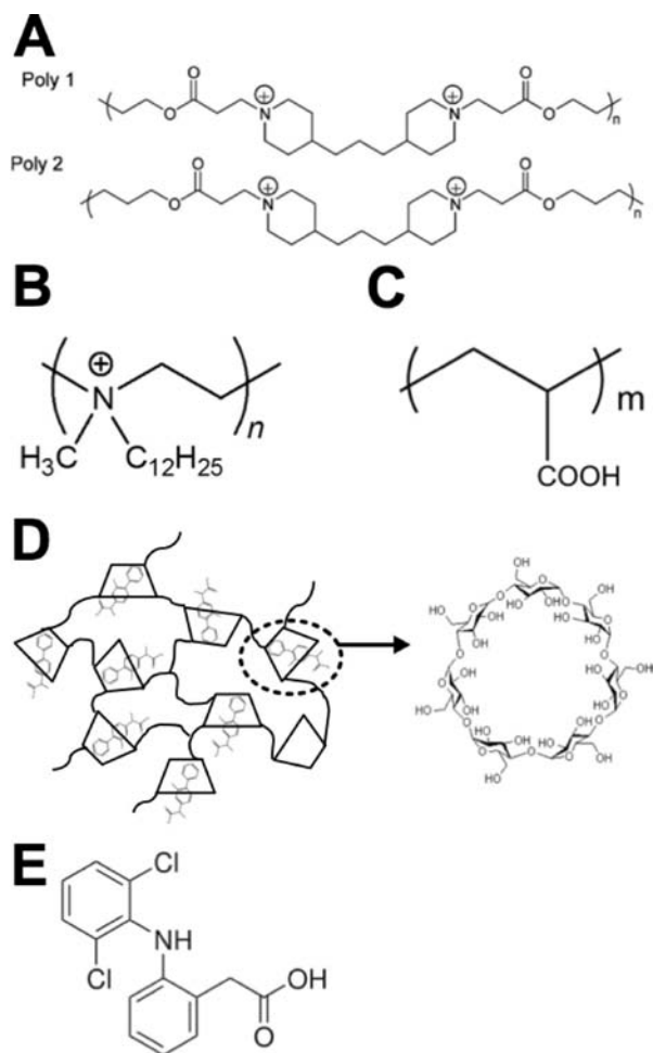
Figure 1. (A) Structure of hydrolytically degradable poly( \beta -amino ester)s, Poly1 and Poly2. (B) Structure of microbicidal linear N,N -dodecyl, methyl-PEI (DMLPEI). (C) Poly(acrylic acid) (PAA). (D) Schematic of poly( \beta -cyclodextrin) with drug sequestered in the interior of its monomer unit, as well as a close-up structure of a monomeric \beta -cyclodextrin. (E) Structure of diclofenac.
